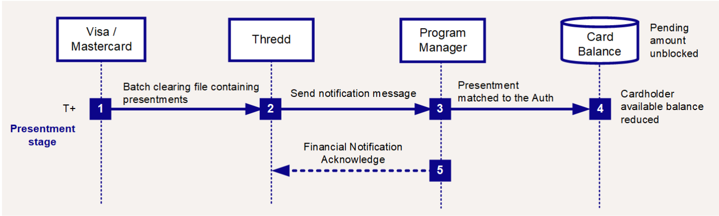
Figure 13: Presentment Flow
