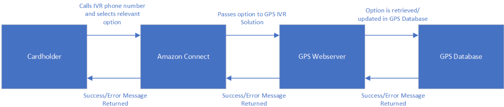
Figure 1: Components in the GPS IVR solution
