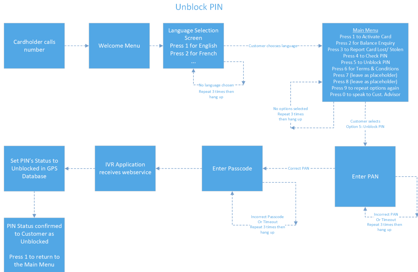
Figure 5: Unblock PIN Example Flow Diagram
